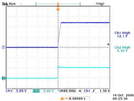
Start-Up Waveform (VIN: 50V, Load: 40A)
