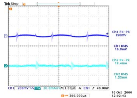
Output Ripple/Noise and Input Ripple Current (VIN: 50V, Load: 40A, LIN=10uH)
