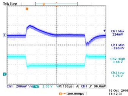
Transient Response (VIN: 50V, Load: 20.0A/10.0A@2.5A/μs)
